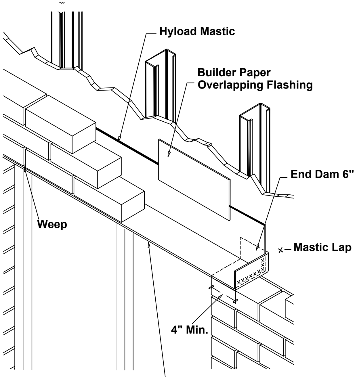
Hyload Surface Adhered w/DRIP Membrane
